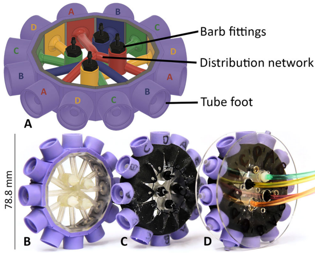
Fig. 5. (A) CAD model of CircleBot which includes four (color-coded) barbed input fittings, and a circular array of tube feet. (B-D) Assembly steps of the CircleBot. (B) A silicone molded linear tube foot array is stretched around a frame. (C) A laser cut nylon sleeve is then placed around the tube feet and thread is used to compress the sleeve to ensure a good seal between the feet and the internal barb fittings. (D) Two 1.5 mm disk wheels are placed on either side of the CircleBot for balance and tubing is installed.
